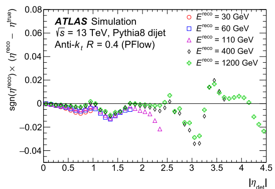
Fig. 6 The signed difference between the reconstructed and truth jet \eta , denoted by \eta^{reco} and \eta^{true} respectively. Each value is obtained from the corresponding parameterized function derived with the PYTHIA8 MC sample and only jets satisfying p_T > 20 GeV are shown
